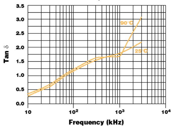
Tan \delta vs. Frequency @ 1.6 mA/cm
