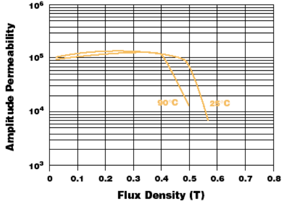
Amplitude Permeability vs. Flux Density @ 10 kHz
