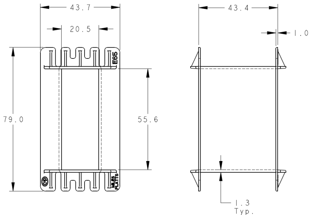
Dimensions in millimeters
