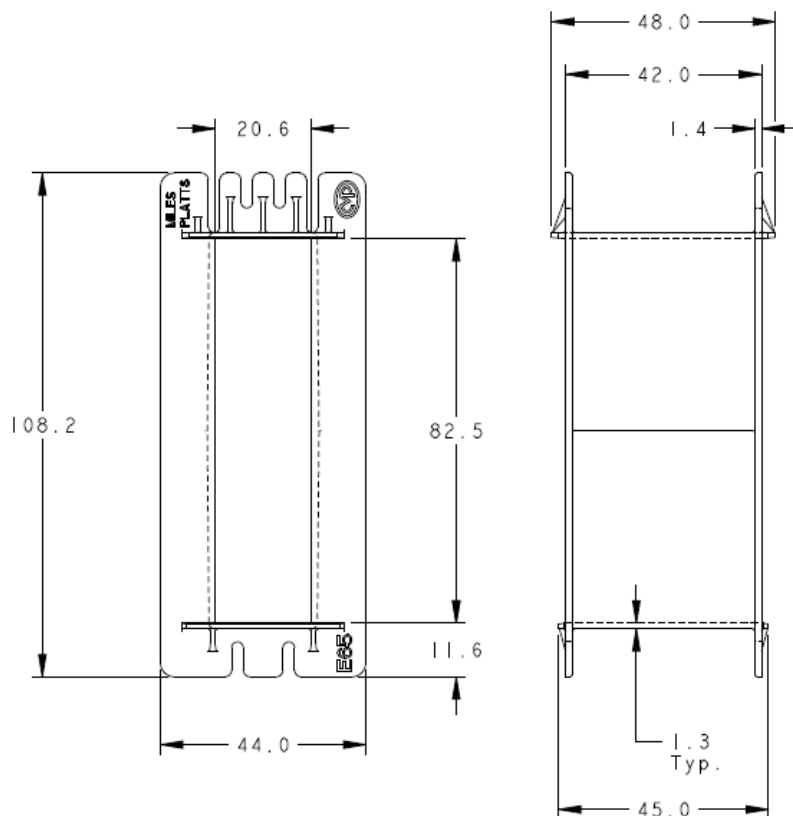
Dimensions in millimeters
