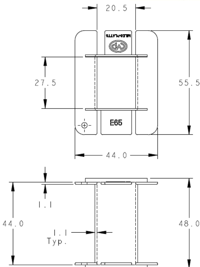
Dimensions in millimeters
